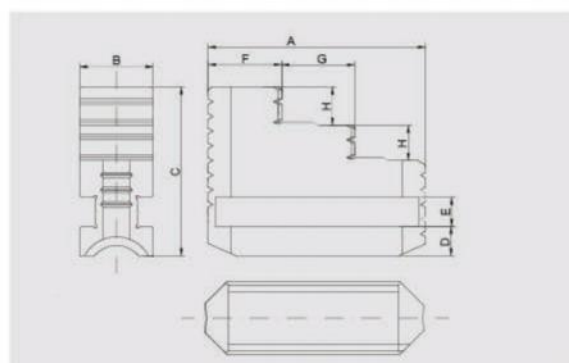
K72卡爪
