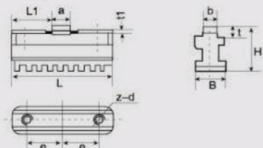
C型分离爪基爪 Two-piece base jaws for form C
