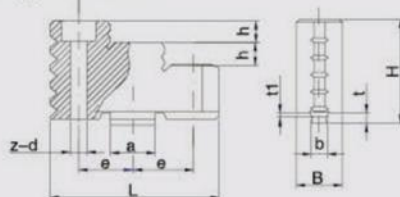
C型分离爪上爪 Two-piece top jaws for form C
