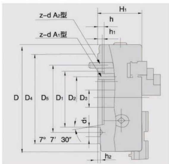
A1型 (内圈螺钉连接) From A1 (Hse inner tapped holes)
